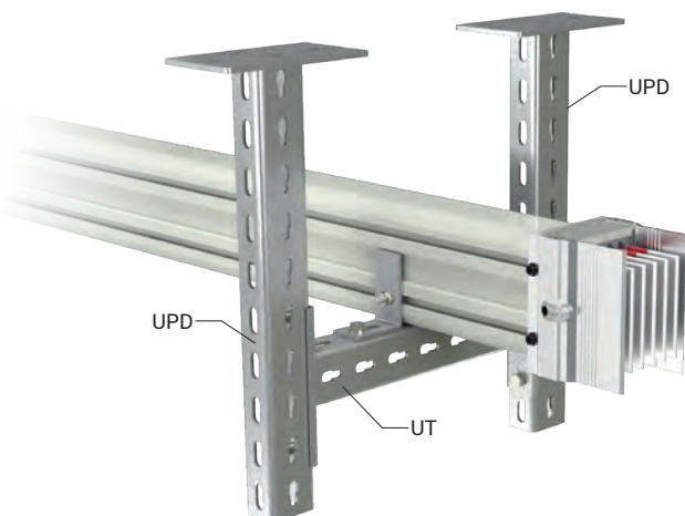
CCR-UT Two-Way For Edgewise Application To UPD Channel
