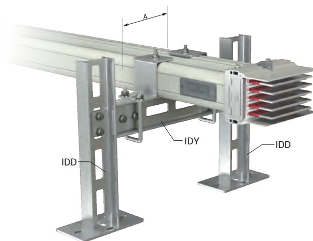
CCR-IDY Two-Way For Edgewise Application To IDD Channel
