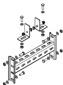
CCR-UT Support Set ("T" bolted)
