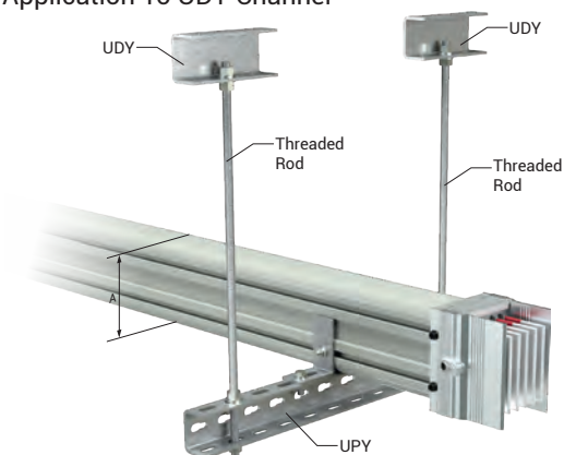
CCR-Threaded Rod Two-Way For Flatwise Application To UDY Channel
