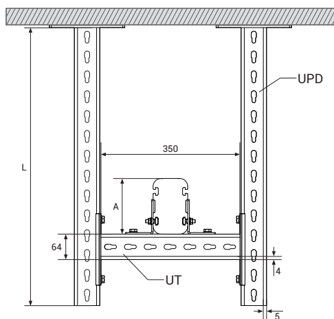
CCR-UT L Support Set ("T" bolted)
