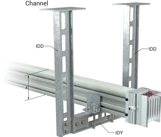
CCR-IDY Two-Way For Edgewise Application To IDD Channel
