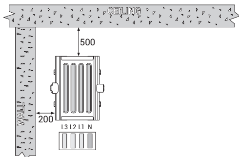
Figure 2 - Edgewise Application
