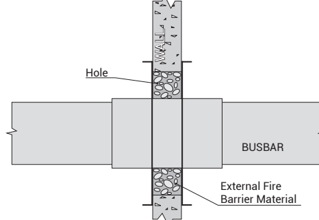
Figure 7 - Standard Wall Crossing
