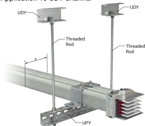
CCR-Threaded Rod Two-Way For Flatwise Application To UDY Channel
