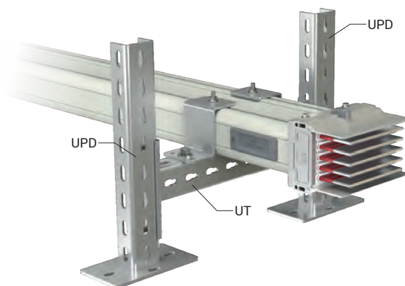
CCR-UT Two-Way For Edgewise Application To UPD Channel
