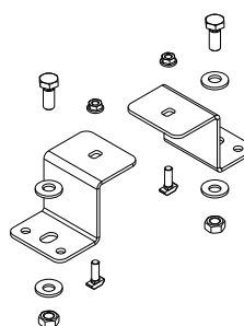
CCR-Z Support Set ("T" bolted)
