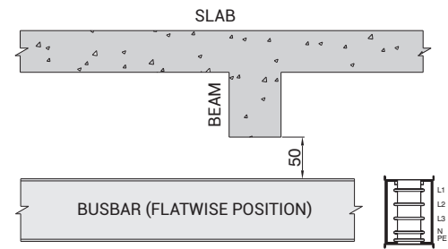
FIGURE-4 SAMPLE WALL CROSSING WITH FIRE BARRIER
