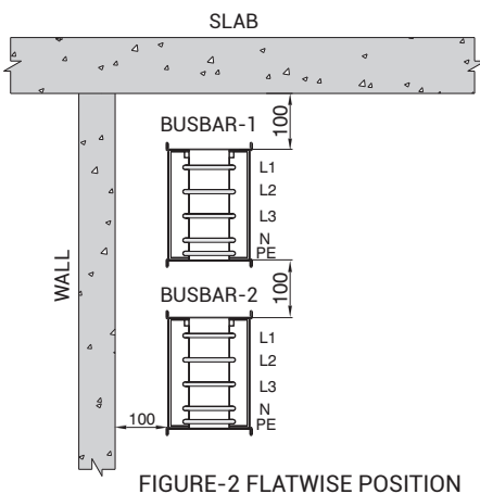
FIGURE-2 FLATWISE POSITION
