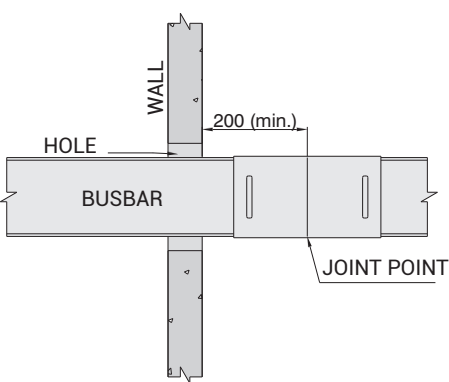
FIGURE-6 STANDARD WALL CROSSING
