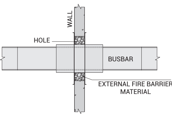
FIGURE-5 SAMPLE WALL CROSSING WITH FIRE BARRIER
