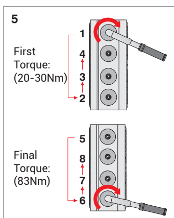
5- If there are more than one bolt for the same phase, bolts shall be tightened by hand approximately 20-30Nm as per above sequence, then 83Nm shall be applied at final torque with the same sequence.
