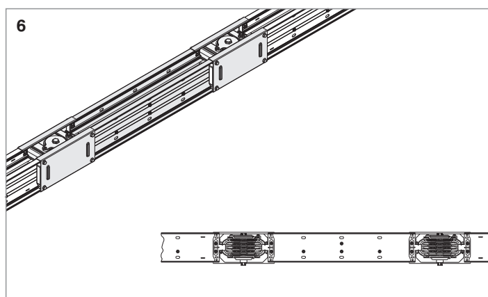
6- Fix the remaining joint cover. Joint installation is completed. (15Nm)
