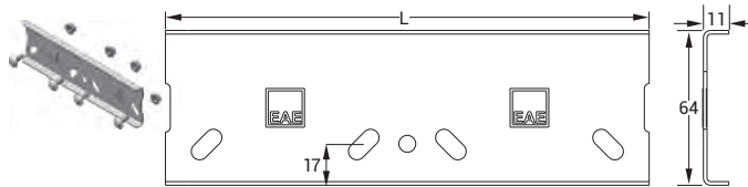
60 CTE Joint Fitting
