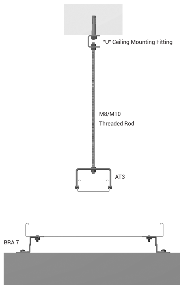
"U" Ceiling Mounting Fitting
