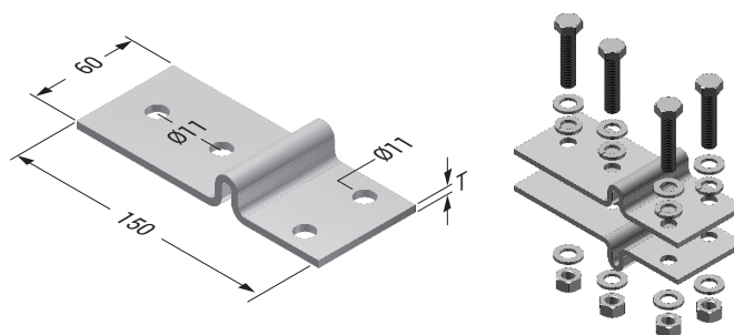
IDK Joint Fitting
